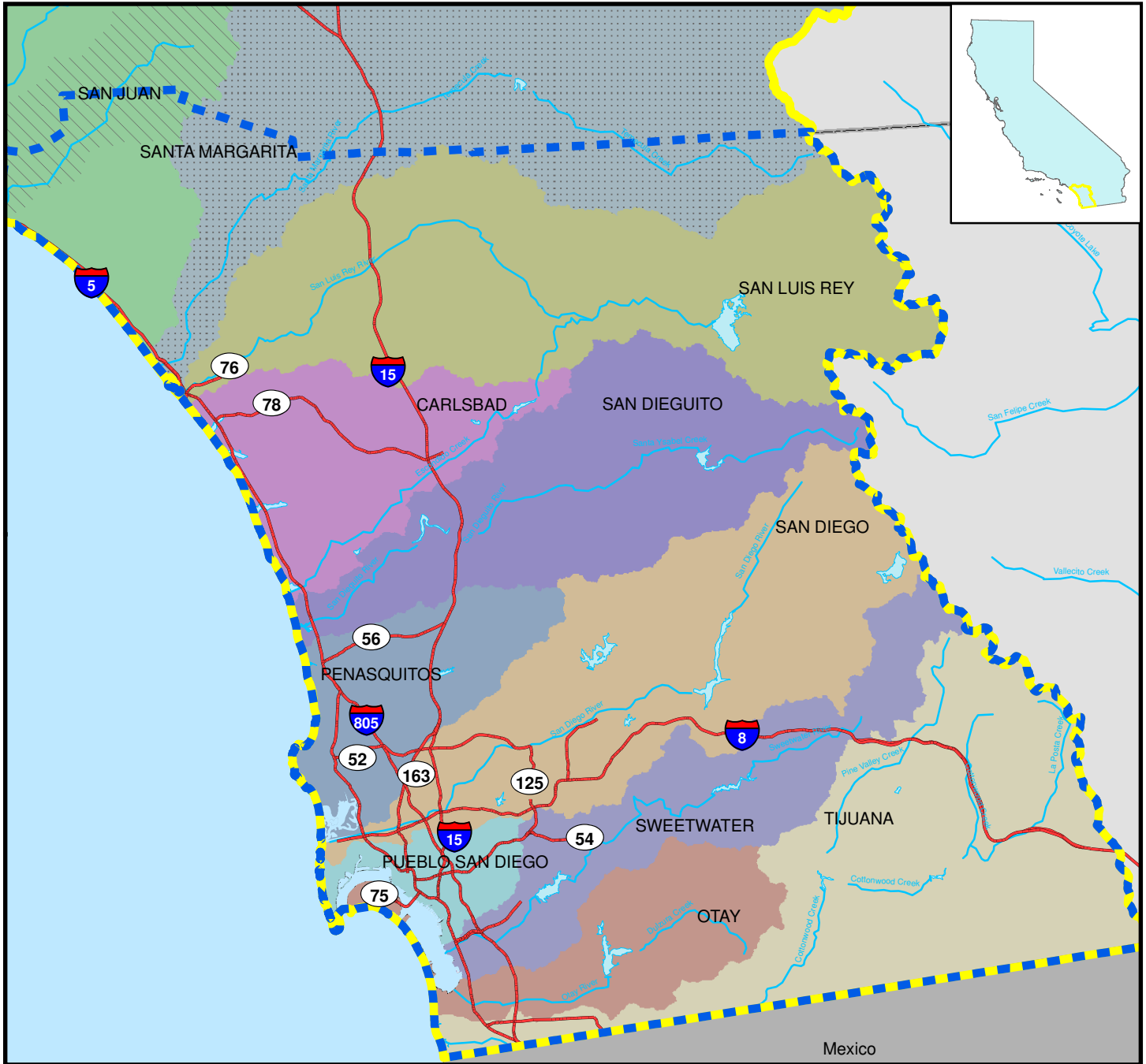
Figure 6-6: Hydrologic Units
